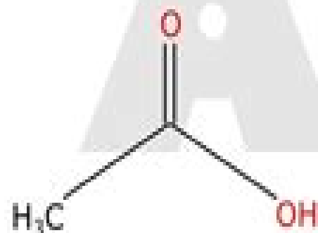
Ethanoic acid
