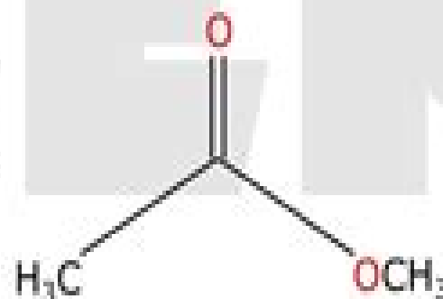
Methyl ethanoate
