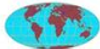
Mollweide Projection
