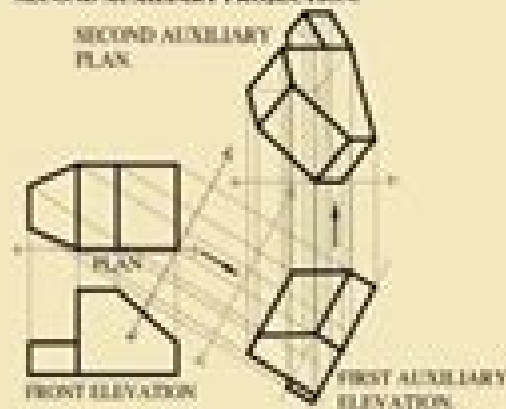
SECOND AUXILIARY PROJECTION.
