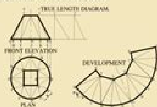
DEVELOPMENT BY TRIANGULATION.
