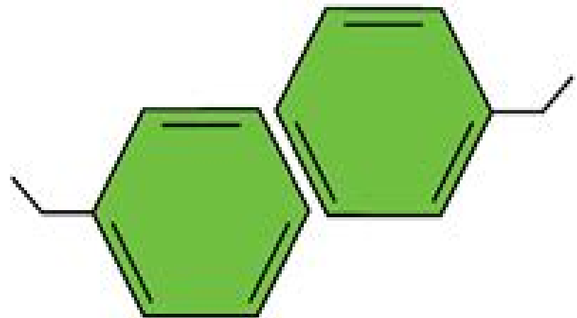
Pi-Pi
