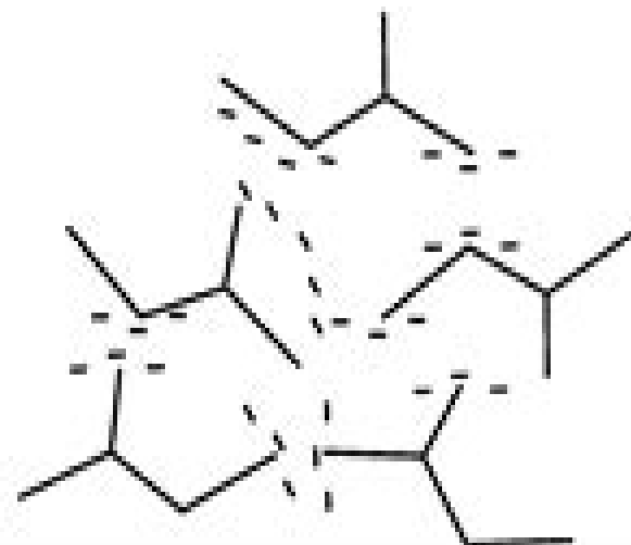
Hydrophobic
