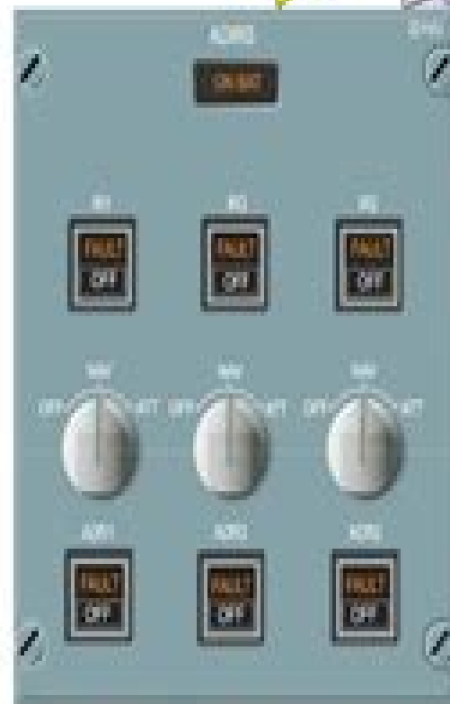
Air Data/Inertial Reference System (ADIRS) Mode Selector Unit (MSU) (221VU)
