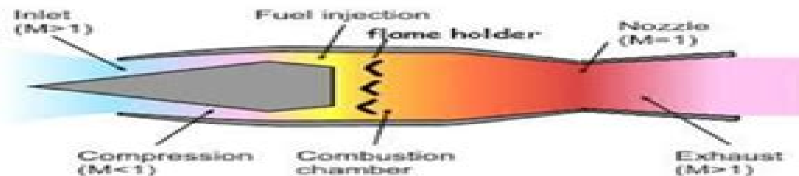
Figure 4.5 ramjet
