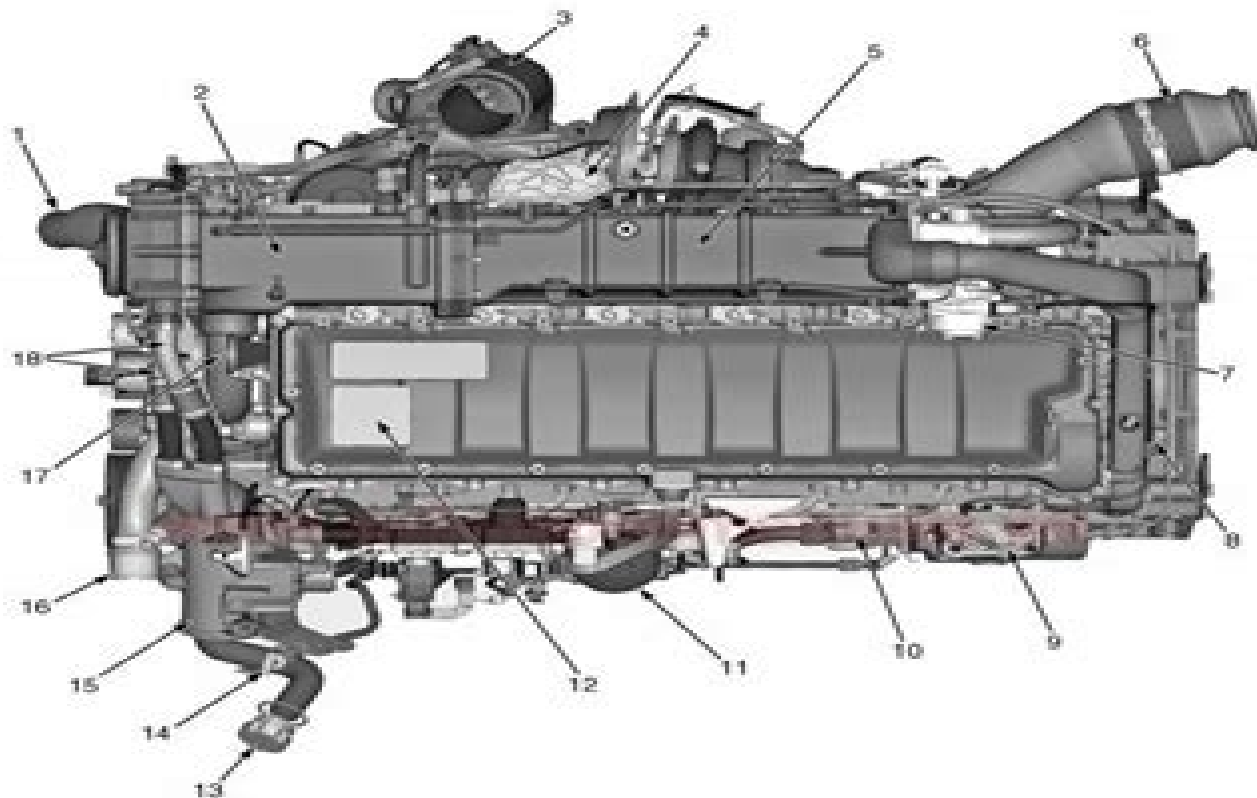
Figure 3 Component location – top view
