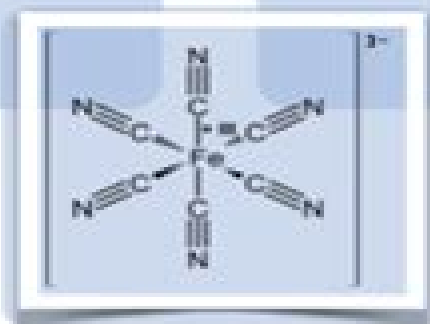
Fig 2: Stereochemistry Table
