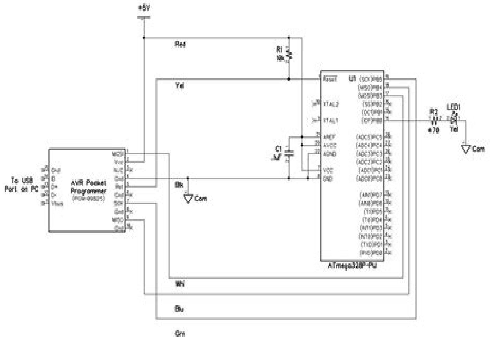
ATmega328P Programming Circuit with AVR Pocket Programmer
